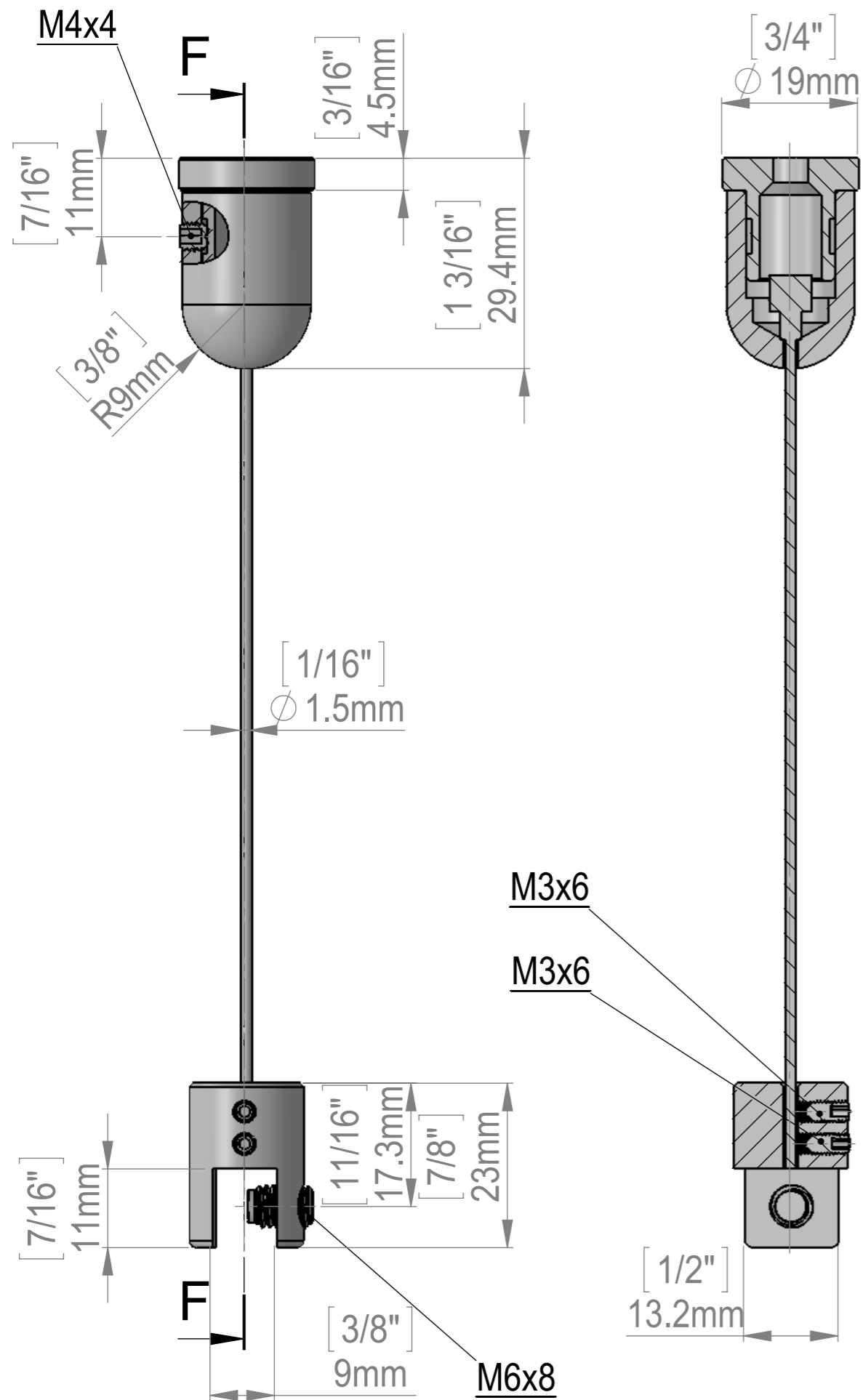
SECTION F-F SCALE 1.3 : 1
