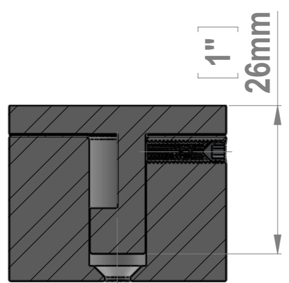
SECTION B-B SCALE 1.5 : 1
