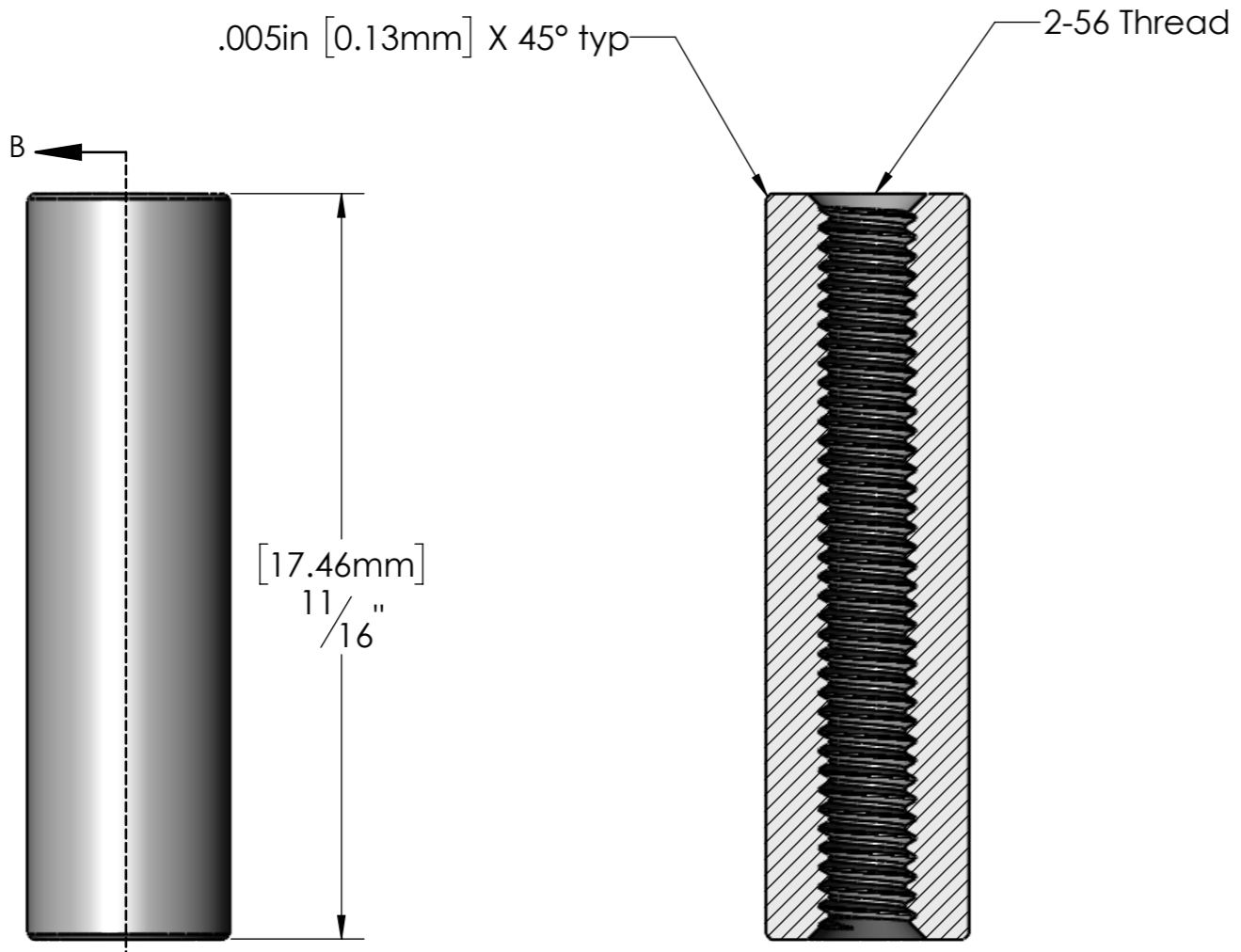
SECTION B-B
