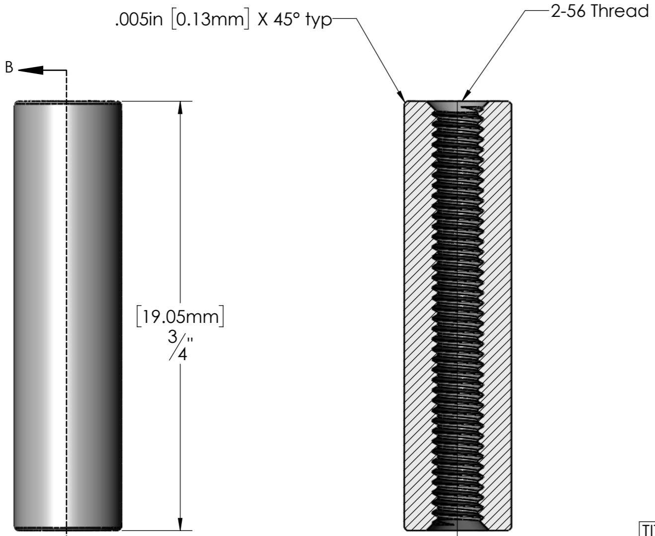
SECTION B-B
