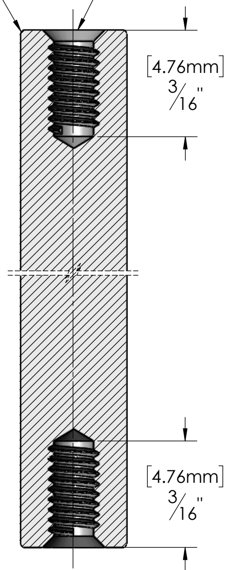
SECTION C-C
