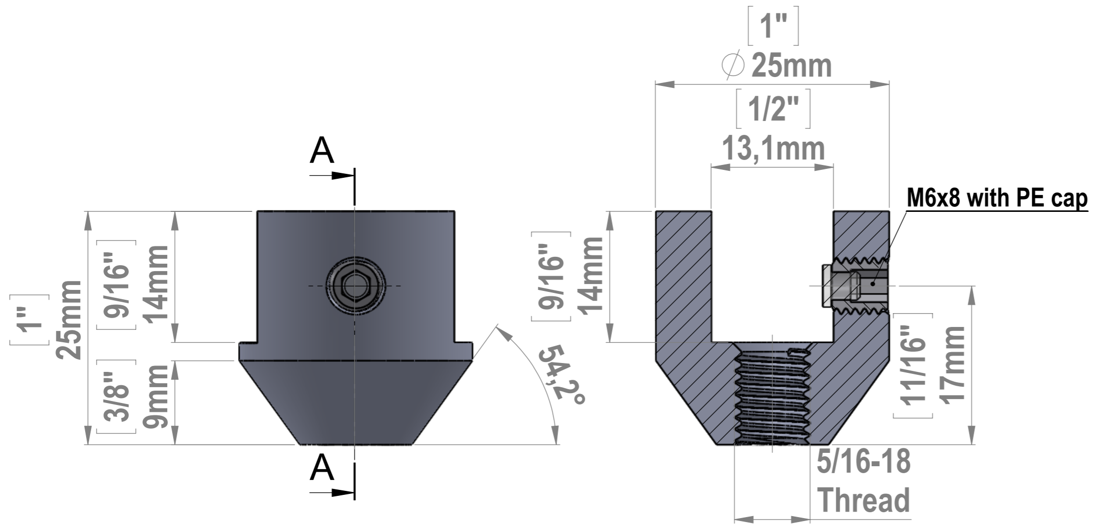
SECTION A-A SCALE 2.5 : 1
