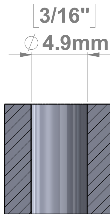
SECTION S-S
