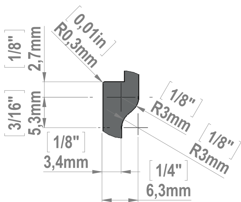
DETAIL B SCALE 3 : 1
